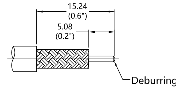
Dimensions in millimeters(inches)
