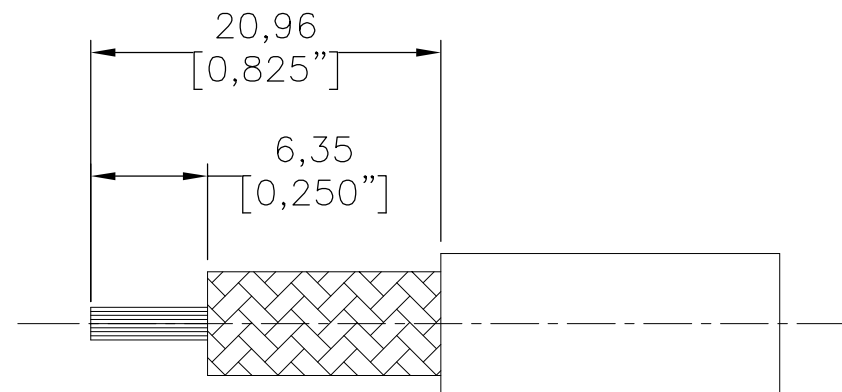
RECOMMENDED CABLE STRIPPING DIM'S Connector Adds: 28.7 mm
