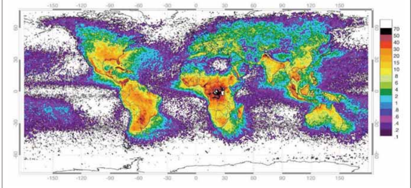
Global distribution of lightning from April 1995 through February 2003 from the combined observations of two NASA instruments.
