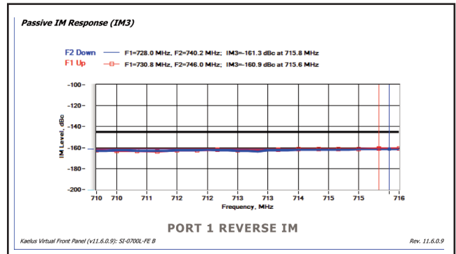
Electrical Performance of 80 ft 7-16 DIN/7-16 DIN Assembly
