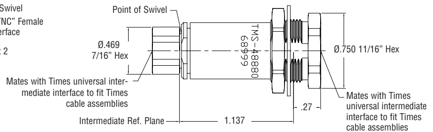
SD48880 In line Rotating Connector
